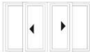
4 DOOR SLIDING DOORS, WIDTH 3000, 3600, 4200. OVERALL HEIGHT 2115 VIEWED FROM OUTSIDE LEFT OR RIGHT HAND FIXED
